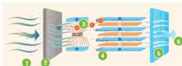
Electrostatic (ESP) Filtration Technology
